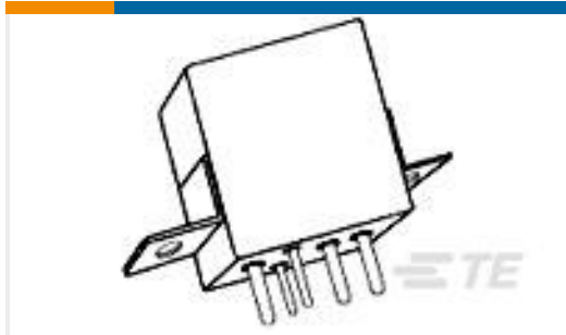
TE Part #2-1617748-3 FCA-125-17=M6106/19-017
