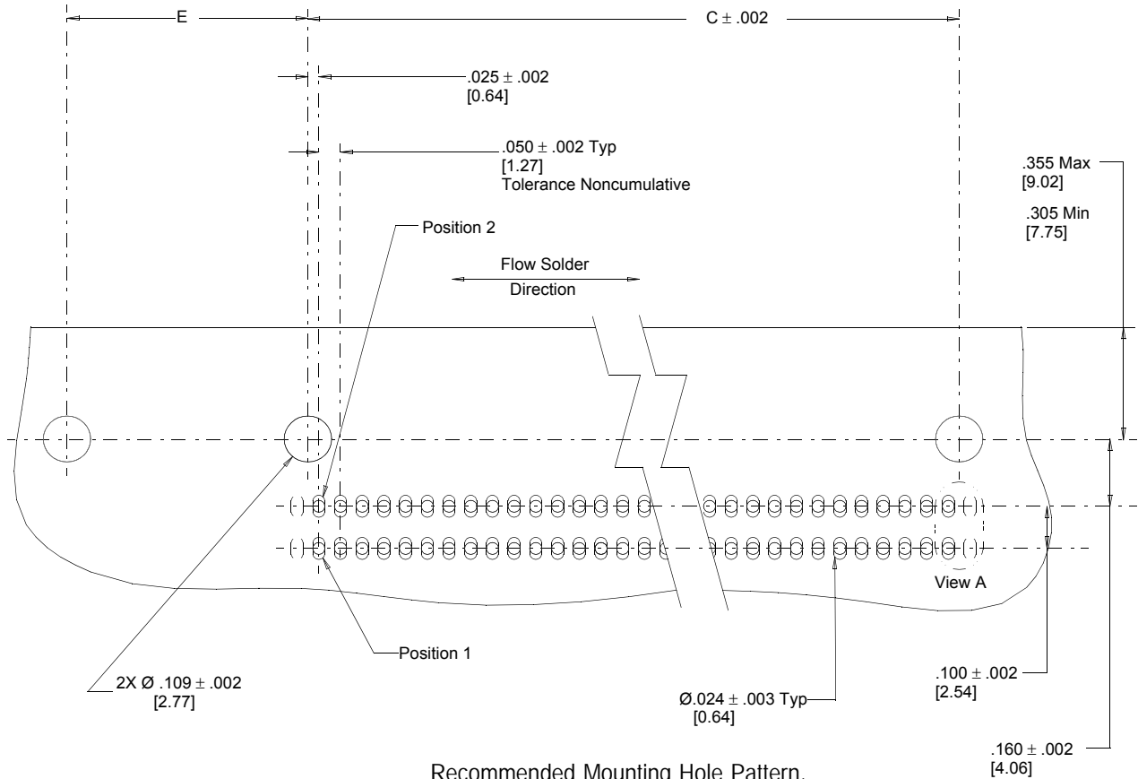
Recommended Mounting Hole Pattern, PTH Right Angle Header
