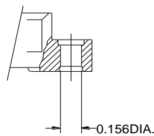
VARIATION 04 .156 +0.002 -0.000 DIA. MOUNTING HOLE
