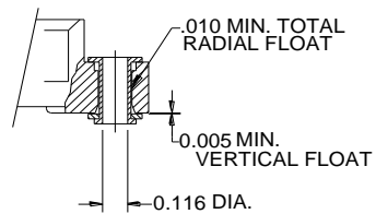
VARIATION 03 .116 +0.003 -0.000 I.D. FLOATING EYELET
