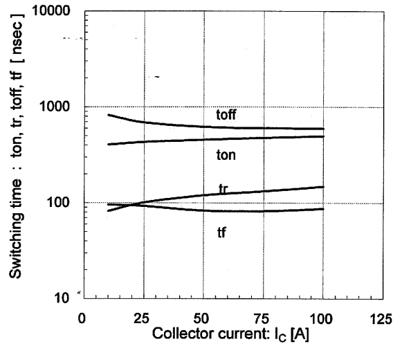
Switching time vs. Collector current (typ.) V_{CC}=600V, V_{GE}=\pm 15V, R_g=15\Omega, T_j=150^\circ C
