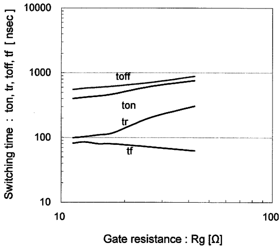
Switching time vs. gate resistance (typ.) V_{CC}=600V, I_c=50A, V_{GE}=\pm 15V, T_j=125^\circ C
