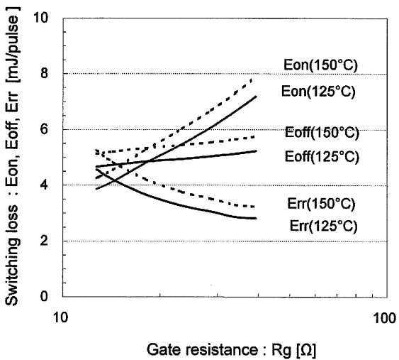
Switching loss vs. gate resistance (typ.) V_{CC}=600V, I_c=50A, V_{GE}=\pm 15V
