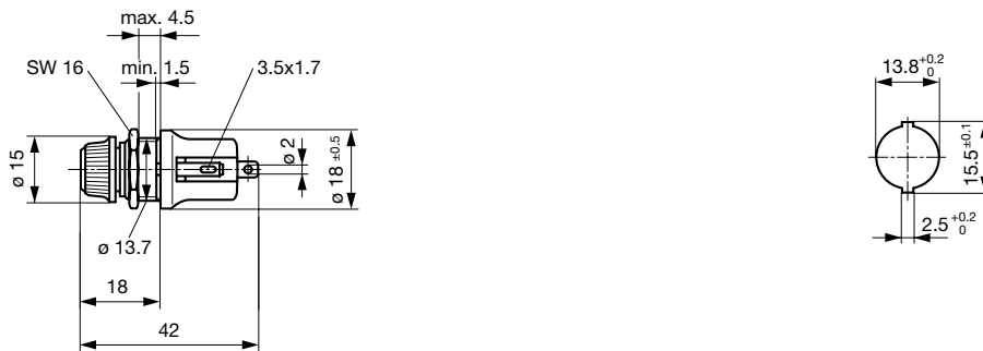
Mounting holes
