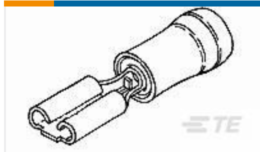
TE Part #165565-6 TERM,RECPT,PIDG,110 FAST,22-16, PHBR,AU
