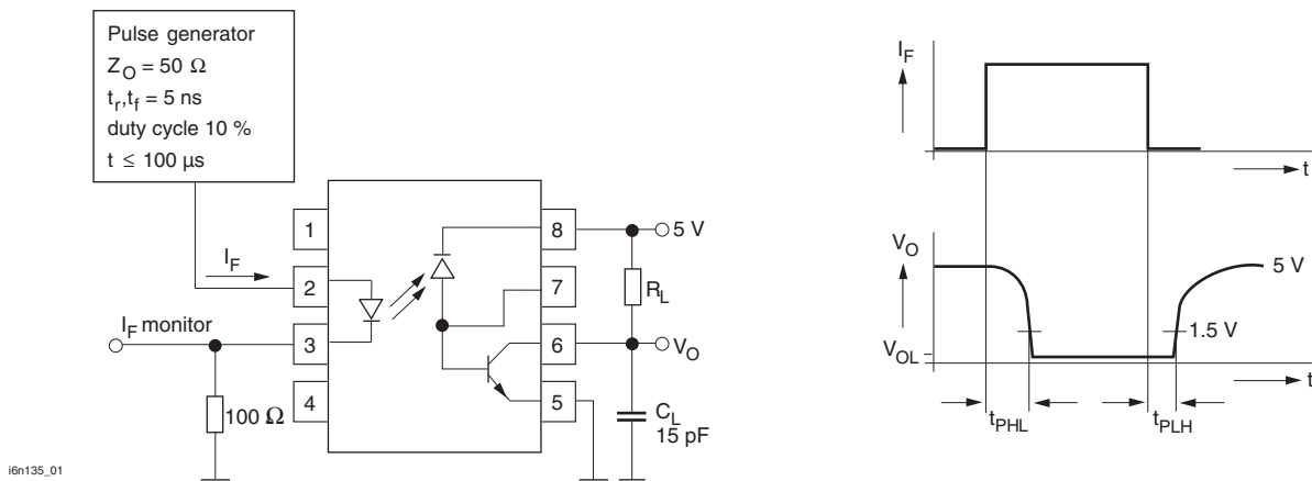
Fig. 10 - Switching Times
