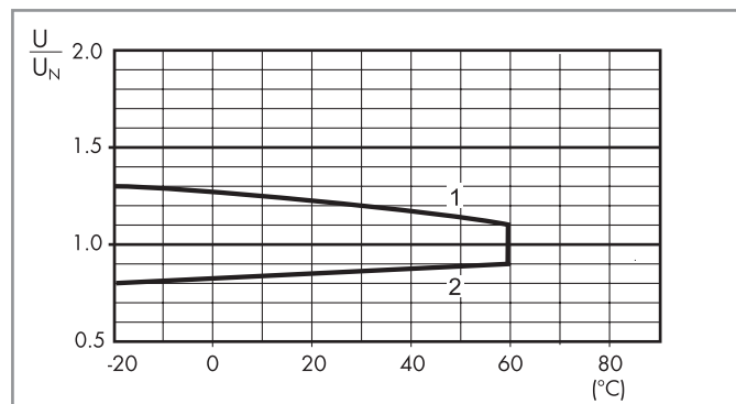
R 67 - Operating range v ambient temperature, 67.xx-x500 with standard (continuous) coil energization (–40...+60)°C
