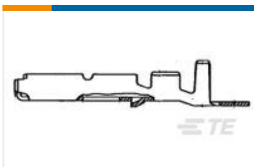
TE Model / Part #172776-2 MIC MK-2 REC CONTACT GOLD
