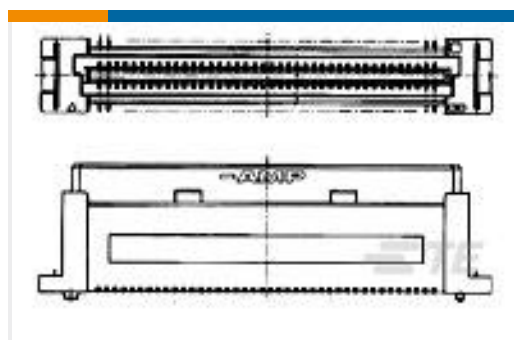
TE Model / Part #1-1939479-3 0.8FH REC ASSY TUBE H13 Au0.76
