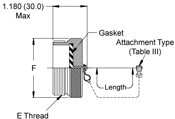
660-023 Plug Cover
