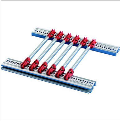
Illustration shows guide rail with 2 end pieces and middle profile
