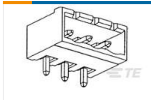
TE Part #796638-4 4POS 5.08MM CE R/A HDR, TRM BLK
