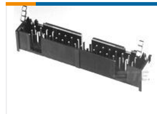
TE Part # 3-1761606-7 IDC LOW PRO HDR 64P VERT LG LA
