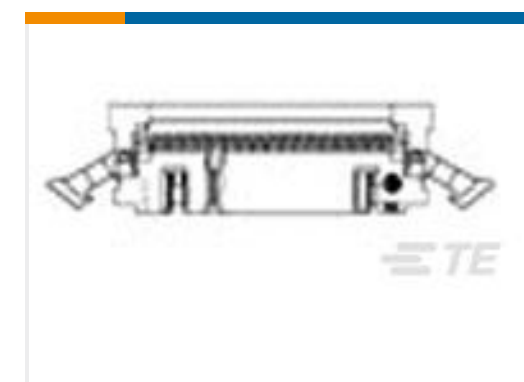
TE Part # 2-111504-6 064 UNIV I/O 30DP NO EARS LTCH
