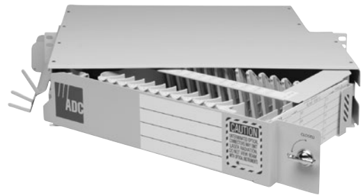
NG3 MicroVAM Chassis
