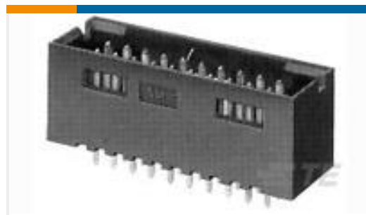
TE Part #5-102619-9 22 MODII HDR DRST SHRD .100CL
