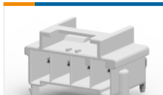
TE Part #1-1969694-4 PTL 1X4 PCB HEADER R/A HITEMP KEY A LGR
