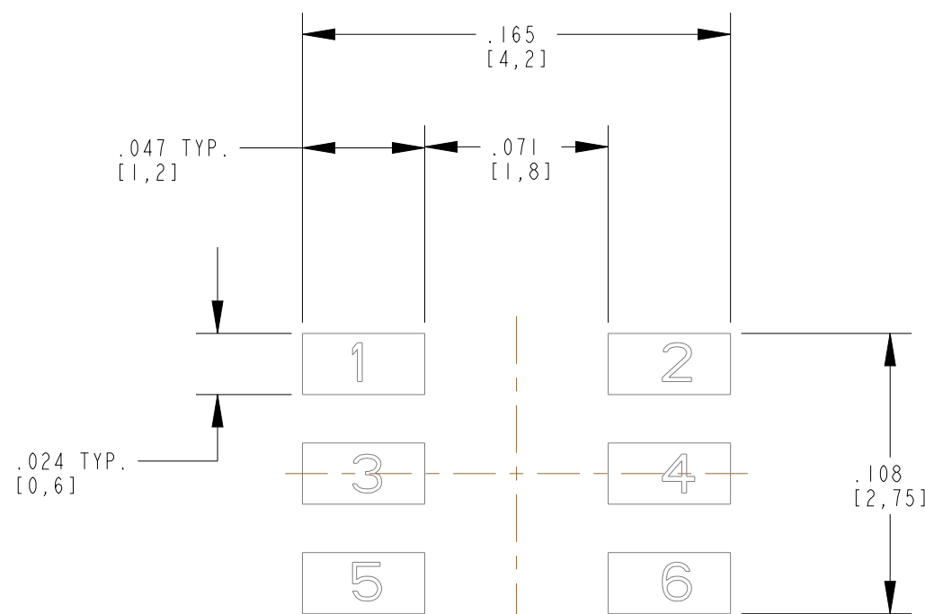
SOLDER PAD LAYOUT
