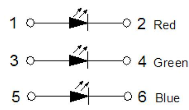
LED SCHEMATIC
