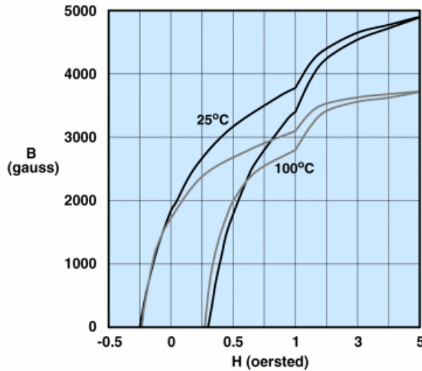
Hysteresis Loop
