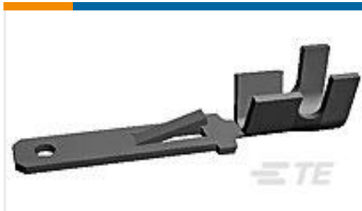
TE Part #42098-2 FF 250 TAB 18-14 AWG PTPB
