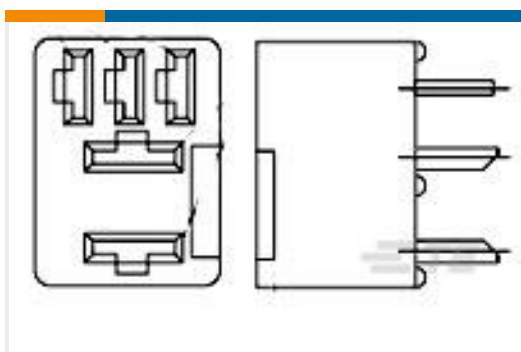
TE Part #1393310-2 VCFM-1000=FROM SEC
