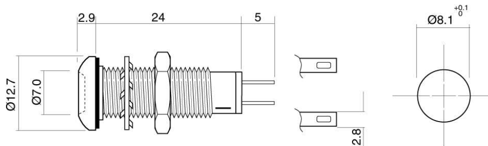
Mounting Hole
