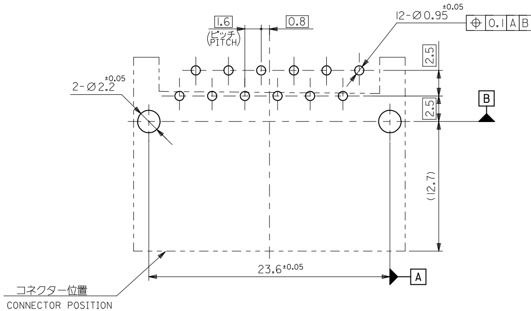
基板取付穴参考寸法 (t = 1.6) RECOMMENDED P.C. BOARD HOLE DIMENSION (REFERENCE) (マウント面) (MOUNTING SIDE)
