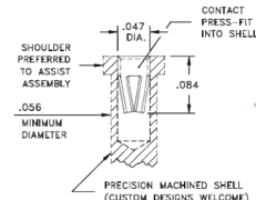
#15 CONTACT FOR .020"-.032" DIAMETER PINS ( \phi = .005 ) 6-FINGER, GROUP K (See page 248)
