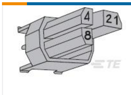
TE Part #6-100525-1 Z-PACK M.CODING KEY
