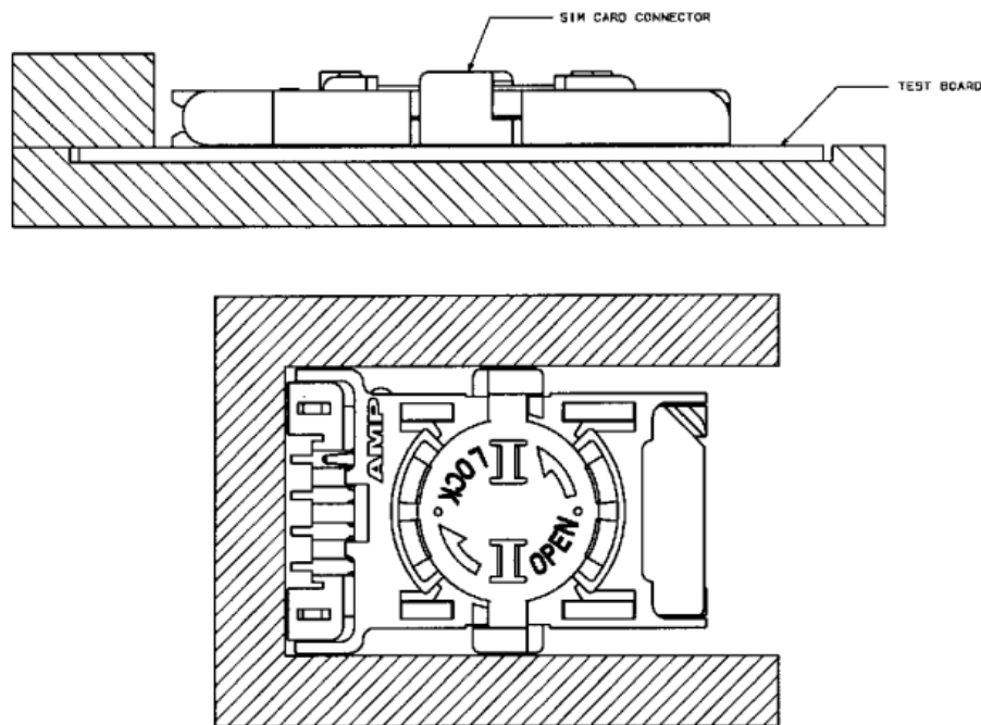
Figure 4 Vibration & Mechanical Shock Mounting Fixture
