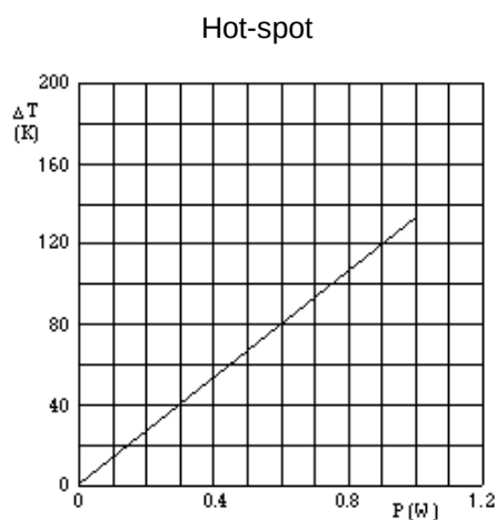
Fig. 1- \phi 0.58mm Cu – leads Hot Spot temperature rise ( \Delta T ) as a function of dissipated power
