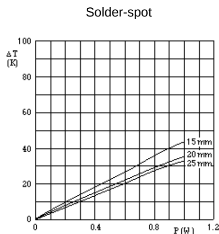
Fig. 2 - \phi 0.58mm Cu – leads Minimum distance from resistor body to PCB=1mm Temperature rise ( \Delta T ) at the lead end (Soldering point) as a function of dissipated power at various leads lengths after mounting.
