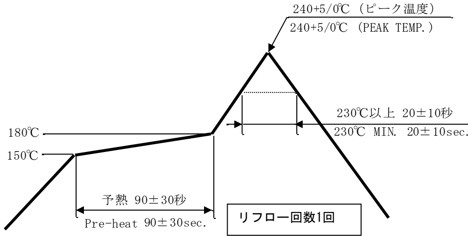
温度条件グラフ TEMPERATURE CONDITION GRAPH
