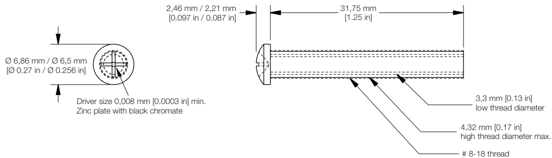
Figure 13. Mounting nut 84508
