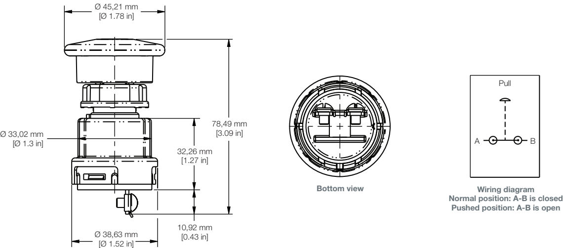
Figure 6. Push-pull/E-stop switches with 1NC circuitry and screw terminal, 90201
