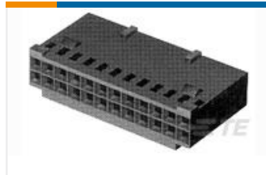
TE Part #2-87631-6 30 MODIV HSG DR MRKD .100 POL
