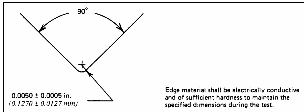
Figure 1. Scrape-Abrasion Edge
