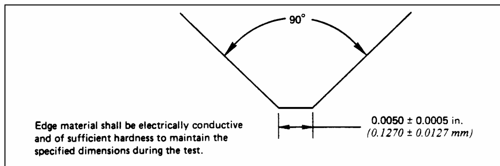
Figure 2. Dynamic Cut-Through Edge
