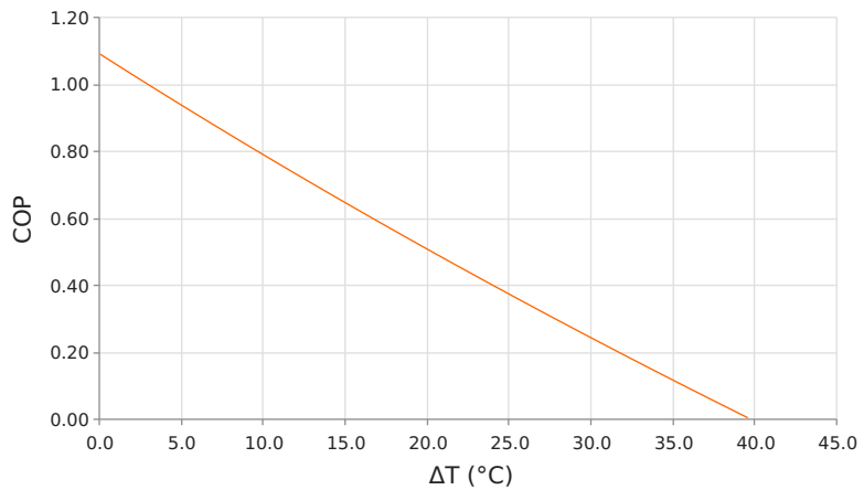
Coefficient of Performance (COP = Qc/Pin) Voperating = 48.1 Volts | Ioperating = 4.4 Amps
