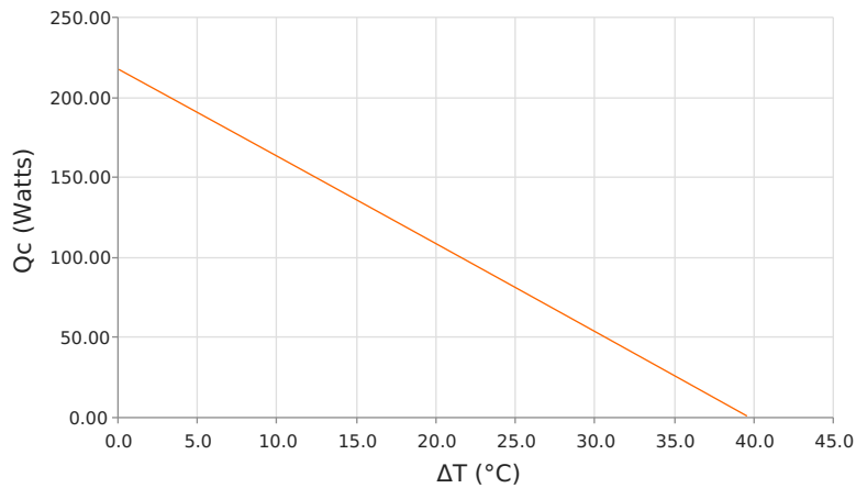
Heat Pumped at Cold Side (Qc) Voperating = 48.1 Volts | Ioperating = 4.4 Amps
