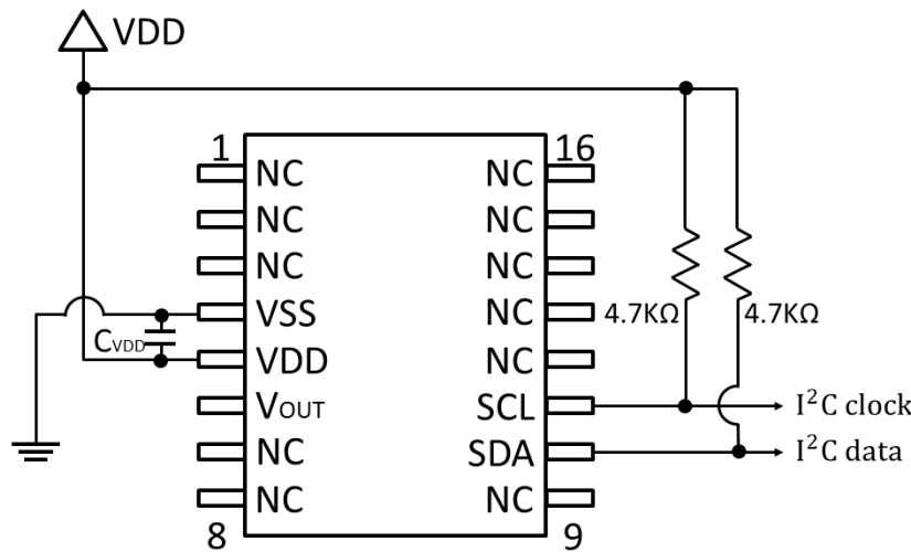
Applications Circuit for SOIC-16 Package
