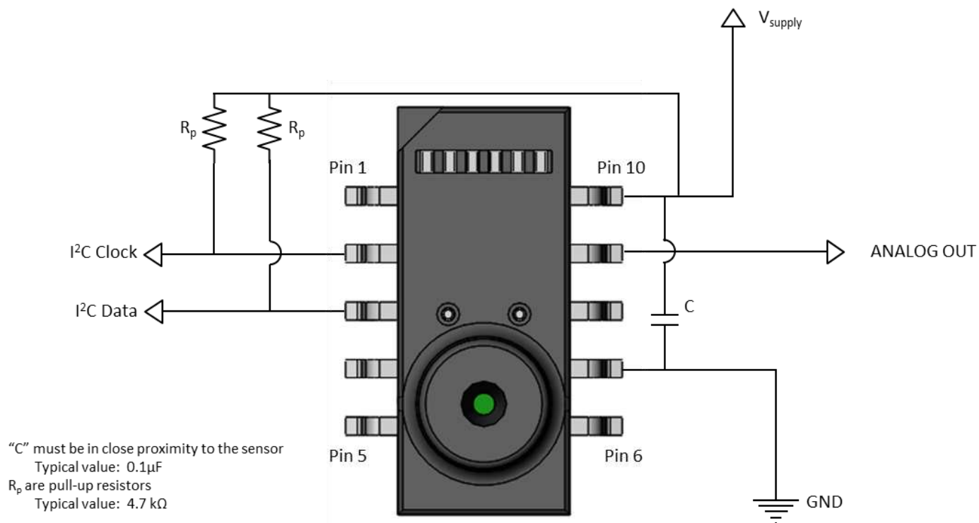
Applications Circuit for SOIC-10 Package
