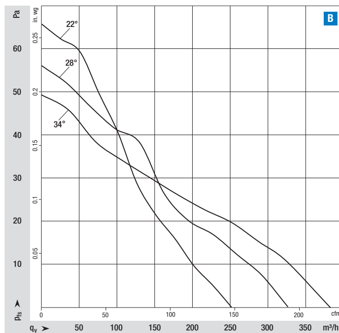
NiQ 3208 with axial blades Ø 172 mm
