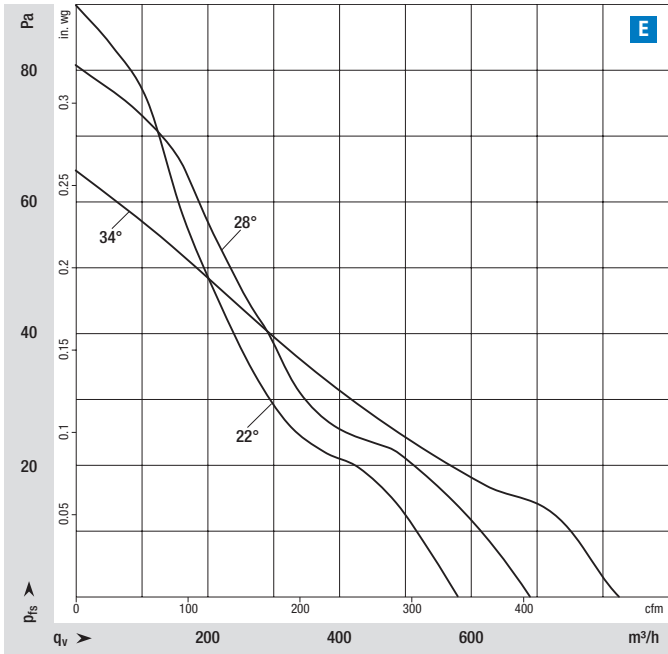
NiQ 3212 with axial blades Ø 230 mm
