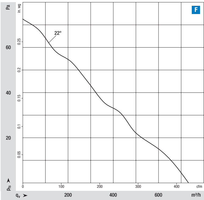
NiQ 3212 with axial blades Ø 254 mm
