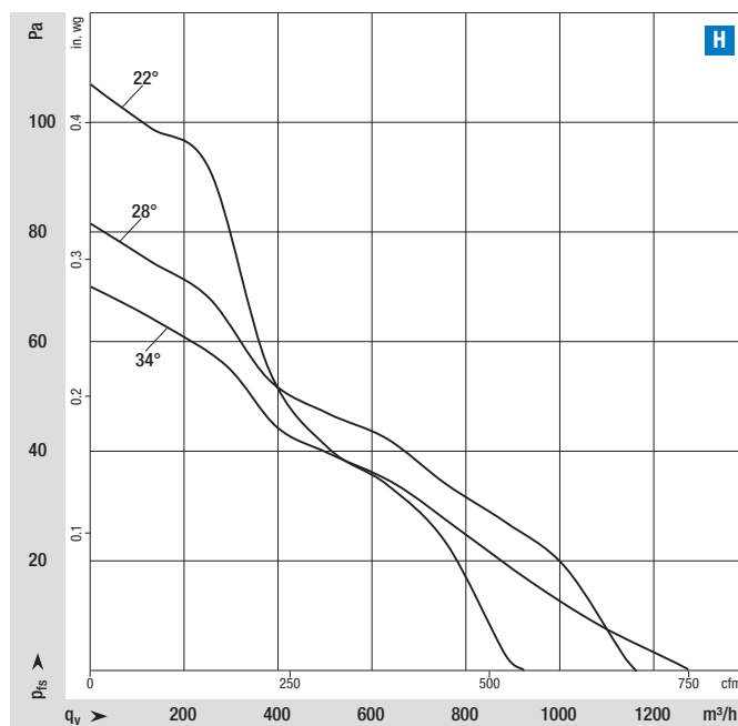
NiQ 3224 with axial blades Ø 254 mm
