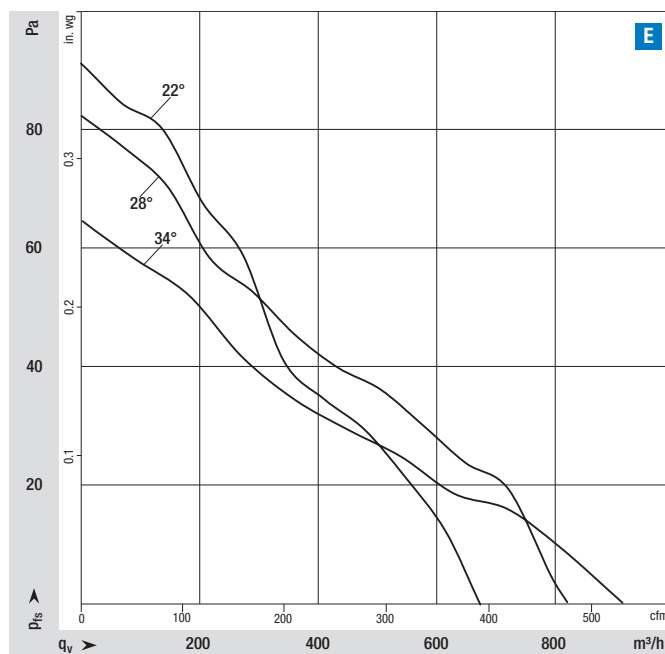
NiQ 3212 with axial blades Ø 230 mm
