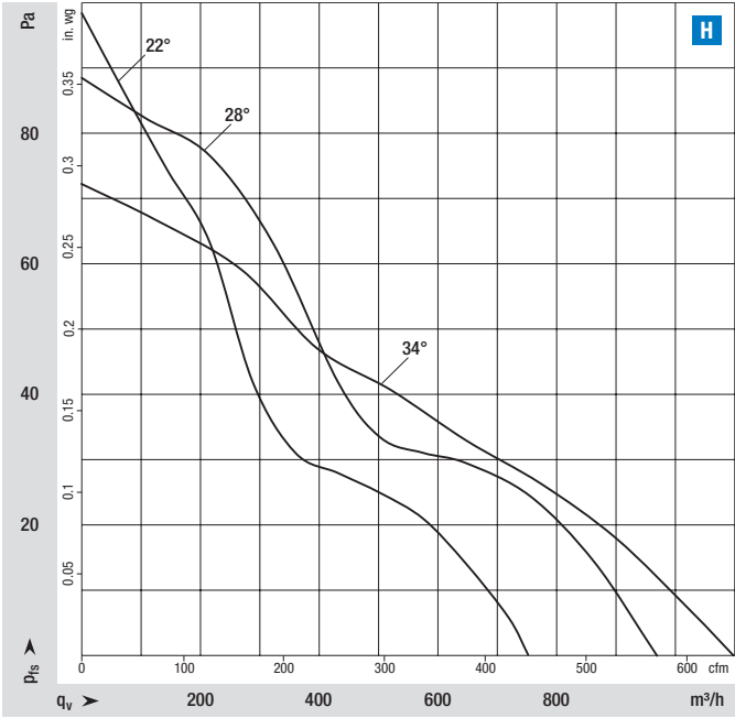
NiQ 3224 with axial blades Ø 254 mm
