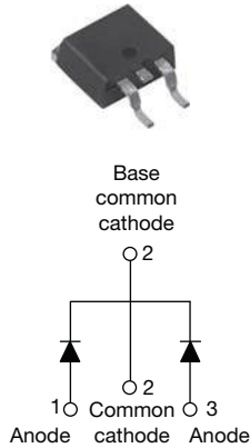
VS-42CTQ030SPbF
