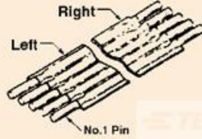
TE Part #2-1474644-7 FSN-21A-4
