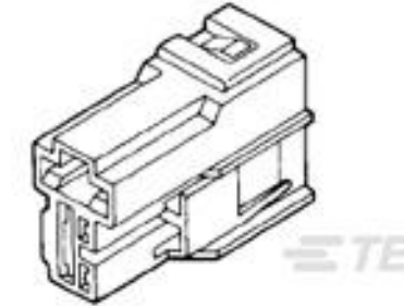
TE Part #172864-2 250 HSG. REC. 6mm 2P BLACK
