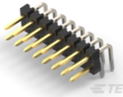
TE Part #1-2842154-0 20P,2MM,BRK HDR,DRRT,2.8,0.1AU, TB W/CAP
