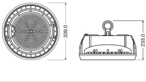
Line drawing of GINO G2 & E Version
