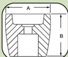
8510 ADJUSTABLE LEG
