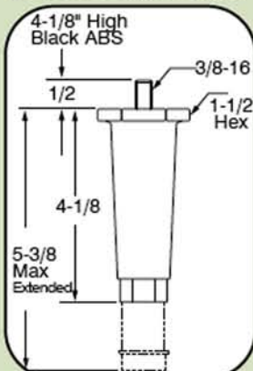
8540 ADJUSTABLE LEG
