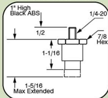
8510 ADJUSTABLE LEG
