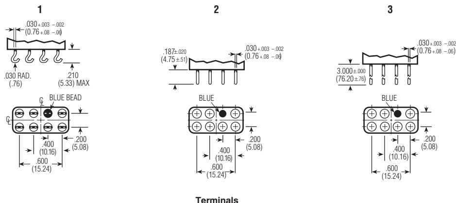
Terminals
