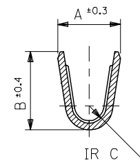
SECT. G-G
