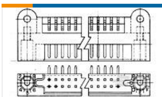
TE Part #530942-2 2 ROW BOX PIN 40 POS R/A
