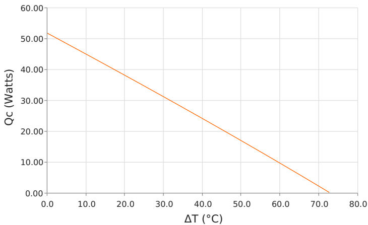
Heat Pumped at Cold Side (Qc) Thot = 85 °C | Current = 5.2 Amps
