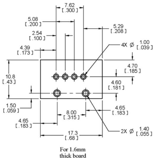
Straight Board Footprint
