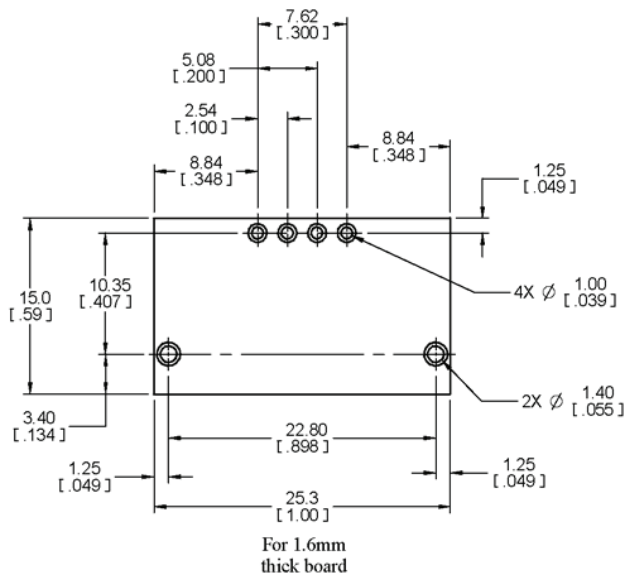
Right Angle Board Footprint
