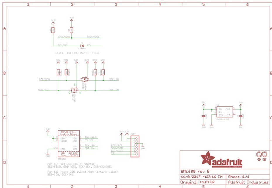
Schematic & Fabrication Print - Original Version
