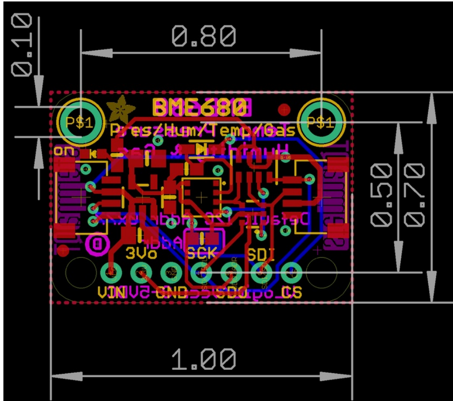
Schematic & Fabrication Print - Original Version
