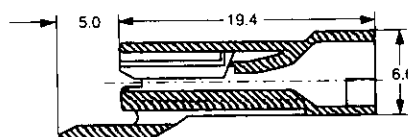
Section X-X
