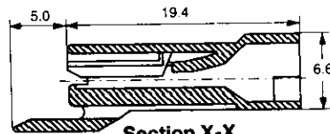
Section X-X
