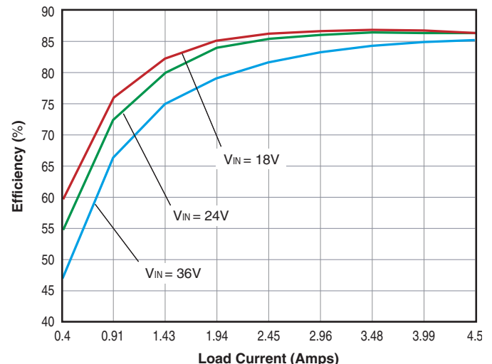
UEP-3.3/4500-D24 Efficiency vs. Line Voltage and Load Current
