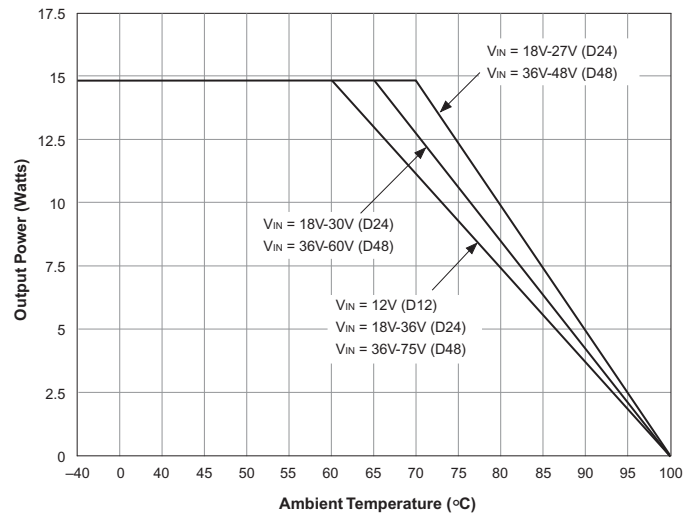
Temperature Derating Curves for UEP-3.3/4500 Output Models
