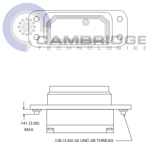
Mounting Style F Cinch Nut Mounting
