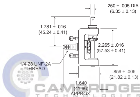
P/N 013837-0001 MA 1/4-28 UNF-2A Thread NOT FOR USE WITH POLARIZING POST
