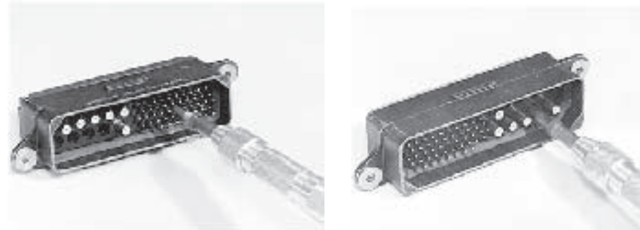
Extracting #20 & #16 Contacts
