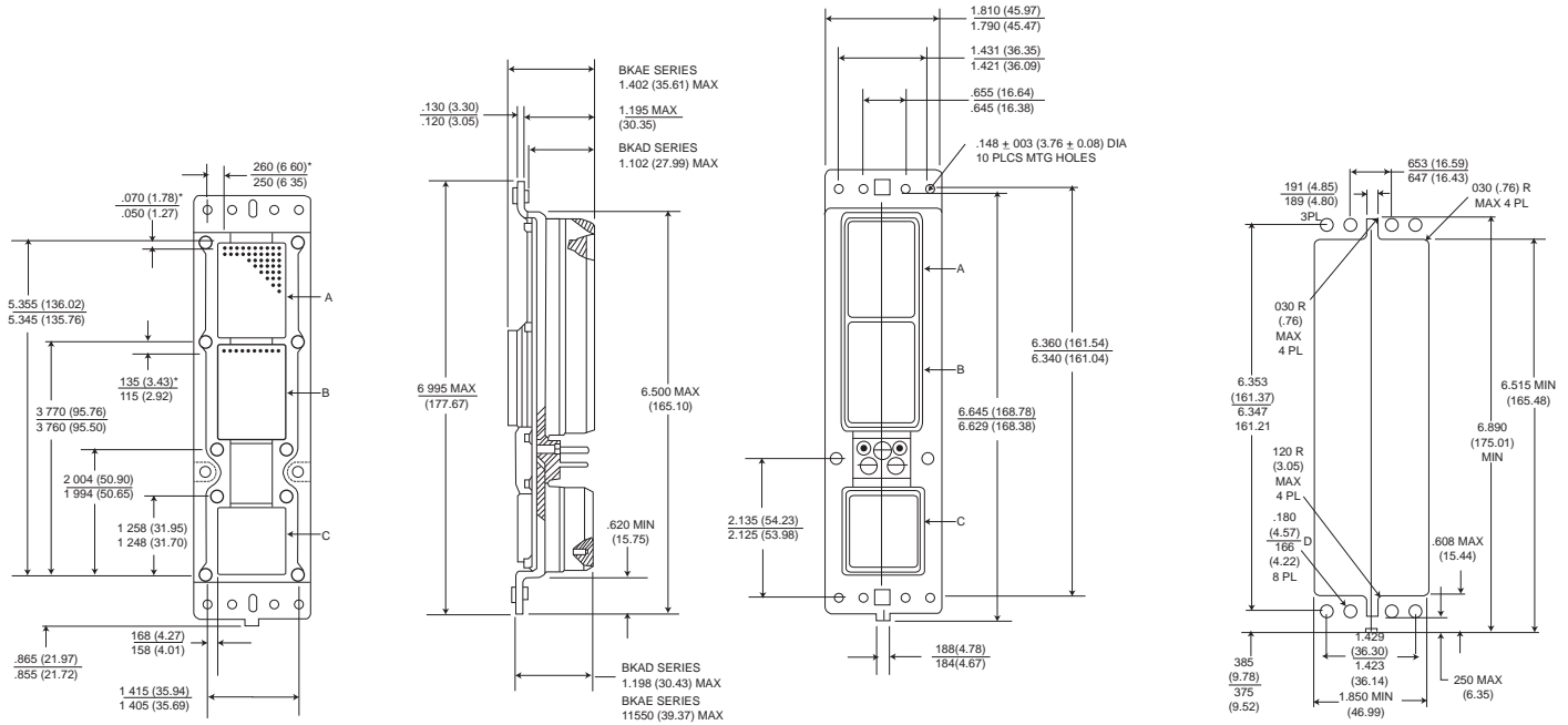
Panel Cutout
