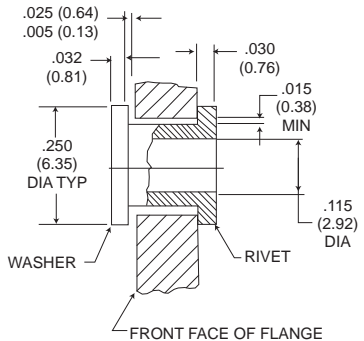
-2301 Modification Floating Eyelets
