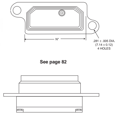
Mounting Style M Mounting
