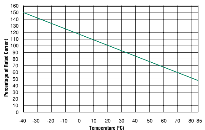
Rating Curve For 3425L Series
