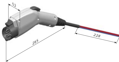
Type I/SAE J1772 Plastic Handle
