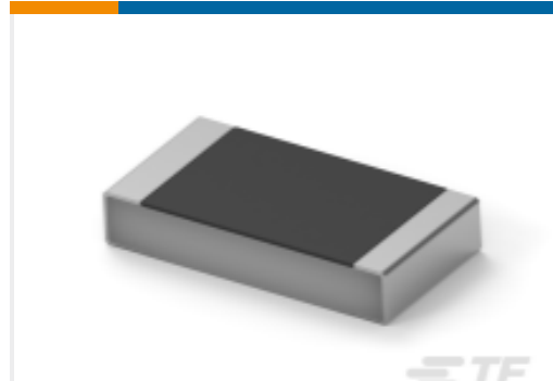
TE Part # 4-2176457-7 CPF 1206 3R01 0.1% 25ppm 5K RL
