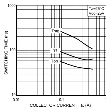
Fig.3 Switching Time
