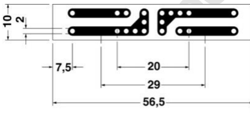
Dimensioned drawing
